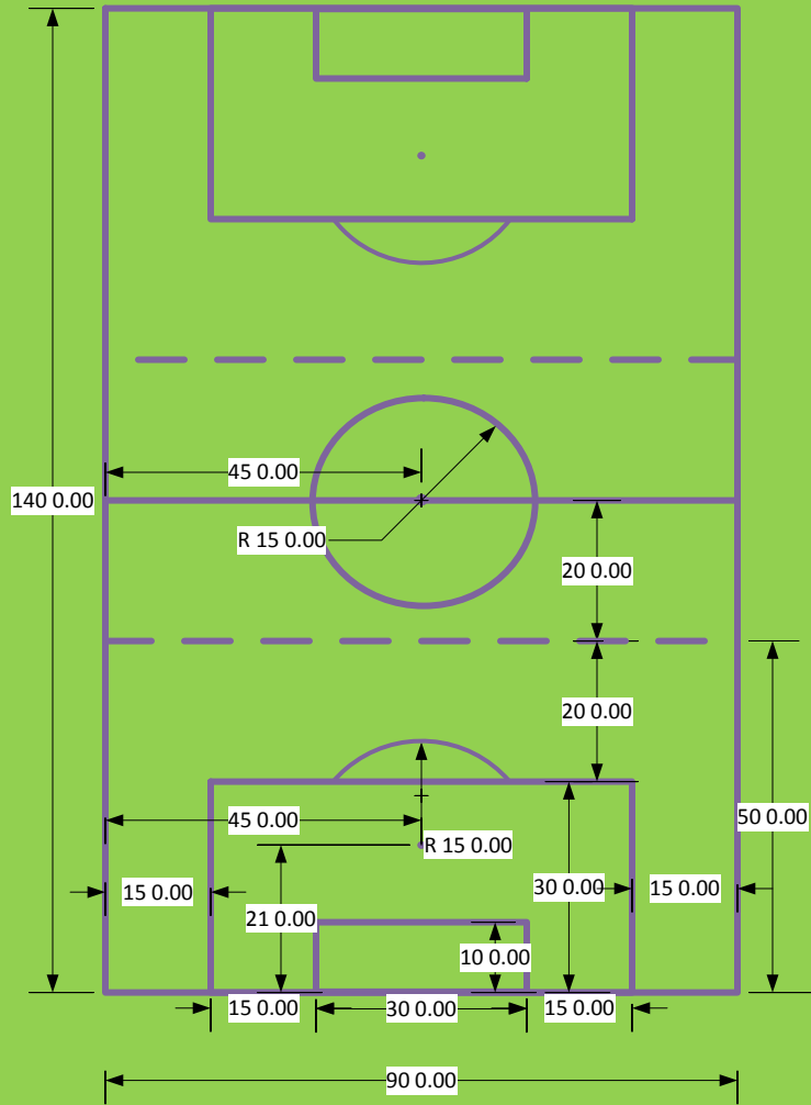
SS Field 1 Dimensions in Feet
