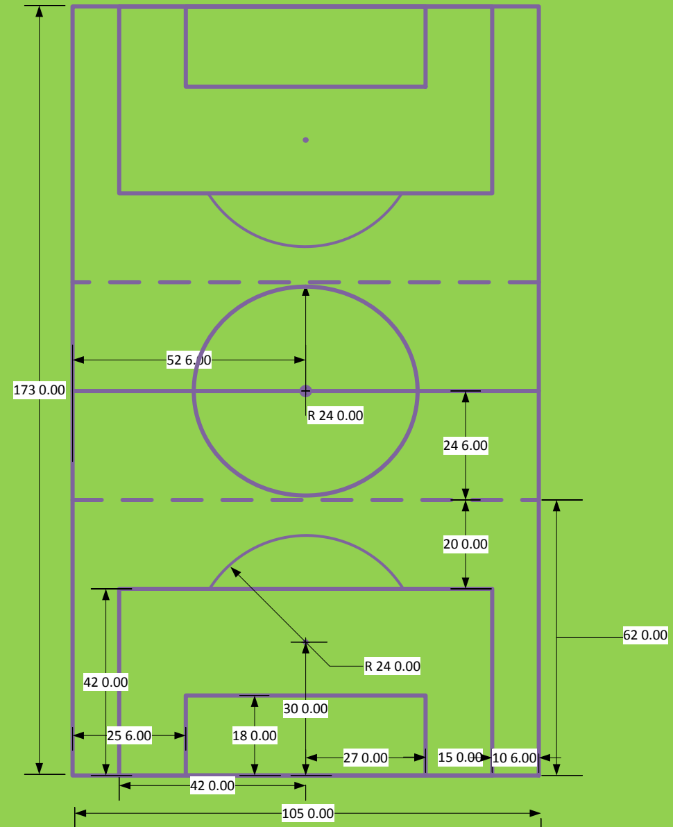
SS Field 2 Dimensions in Feet
